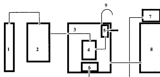
Figure 1. Home made apparatus for extraction with \text{scCO}_2 : 1: \text{CO}_2 reservoir; 2: cryogenic pump (Carlo–Erba SFC 300); 3: thermostatic oven (Carlo–Erba SFC 3000); 4: reactor; 5: six-way valve; 6: alternating field magnetic stirrer; 7: magnetic stirrer control unit; 8: restrictor and oven temperature control unit (Carlo–Erba ICU 600); 9: restrictor
